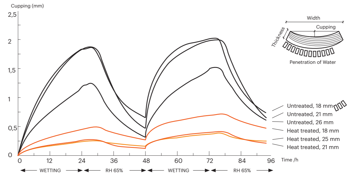
Cupping of exterior cladding boards: Comparison between LunaThermo-D and untreated Scandinavian pine and spruce in different thicknesses.
